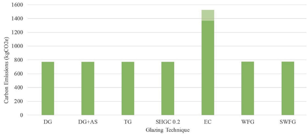
Fig. 6. A4-A5 Stages of LCA ('Gate to Practical Completion'): A4 (Transportation to site), A5 (Construction).
