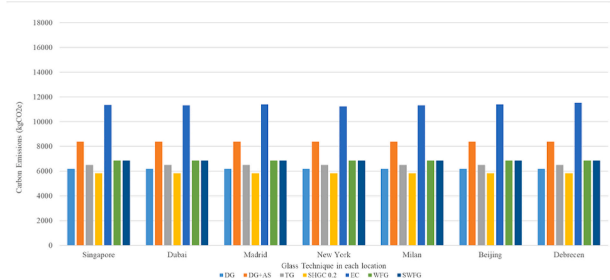
Fig. 7. Use stage, embodied carbon for specific structural elements (B1-Use), B2(Maintenance), B3 (Repair), and B4 (Replacement)).
